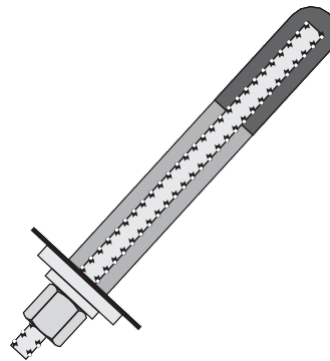
Tensioned fully grouted
