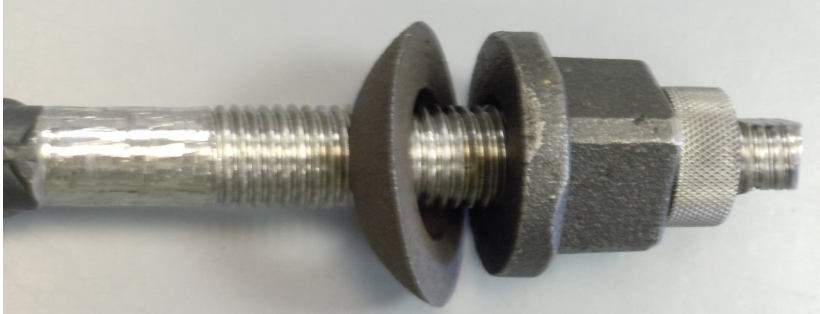
#6 Rebar with 3/4 Flange Nut, Stop Nut and 2" Spherical Washer
