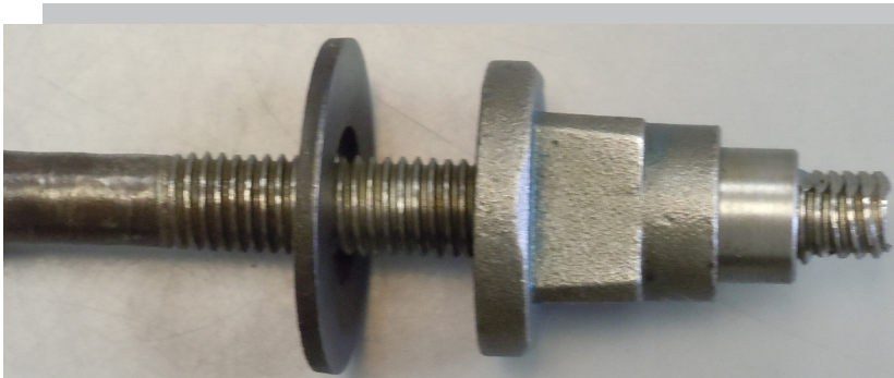
#5 Rebar with 5/8 Chimney Nut, Stop Nut and 2" Washer
